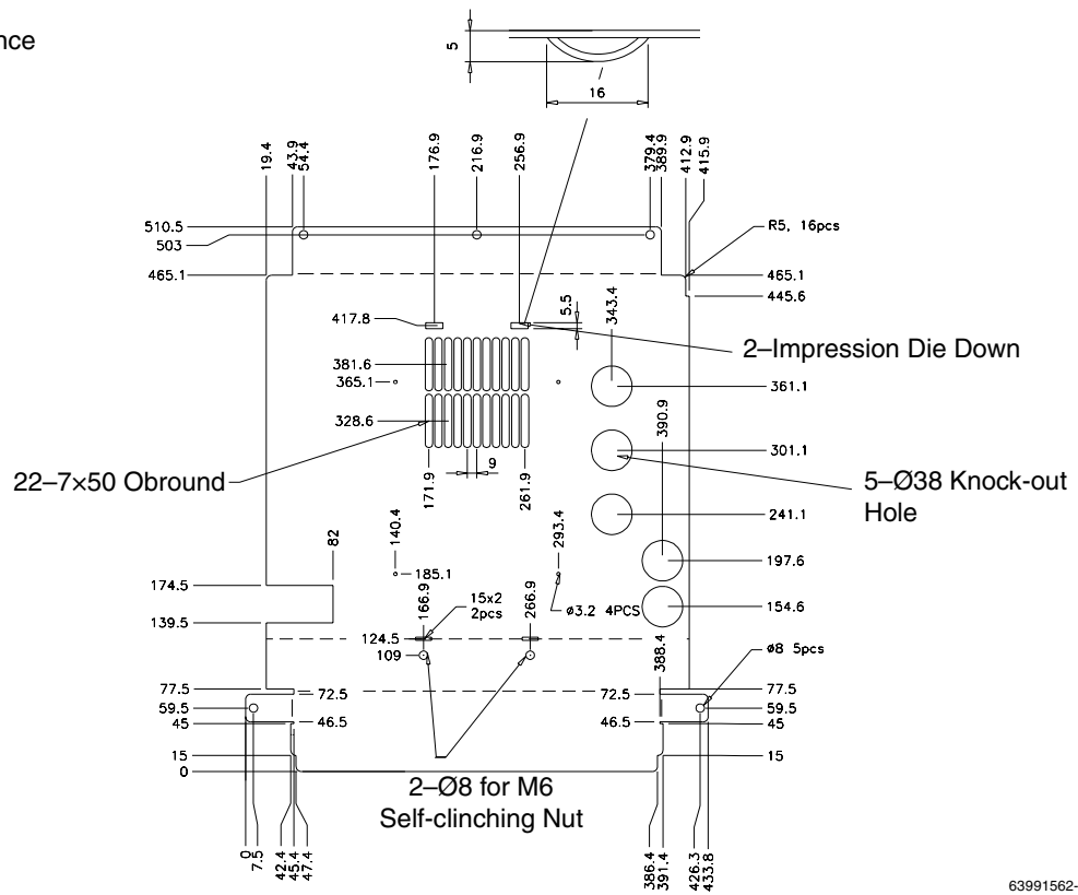
Figure 2-68 Mounting plate for chopper cooling fan.
