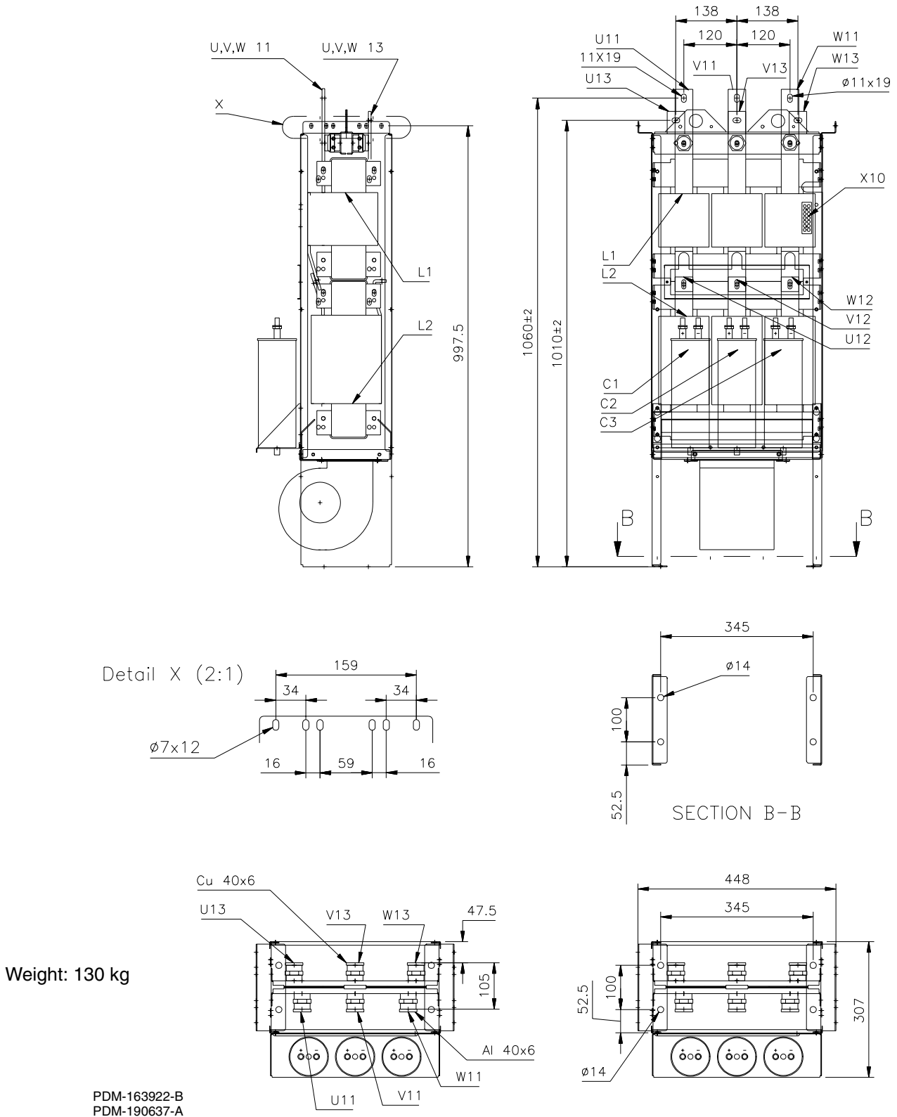
Figure 2-22 ISU_LCL_xR8 dimensions, fixing points and connectors.
