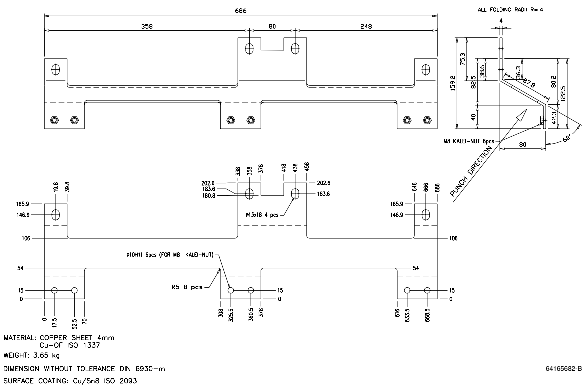
Figure 2-54 The DC busbars (top: +; bottom: -) connecting the R10i/ R11i phase modules. (See Figure 2-55 for the dimensions of the insulator piece.)
