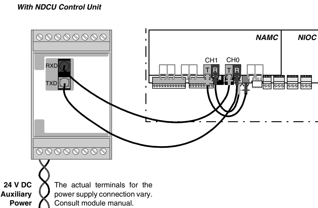
Figure 3-7 Connection of a type Nxxx fieldbus adapter module to the control unit.
