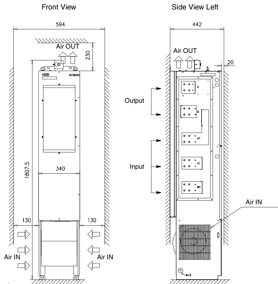
Figure 2-8 Frame B4 supply module dimensions and clearances.
