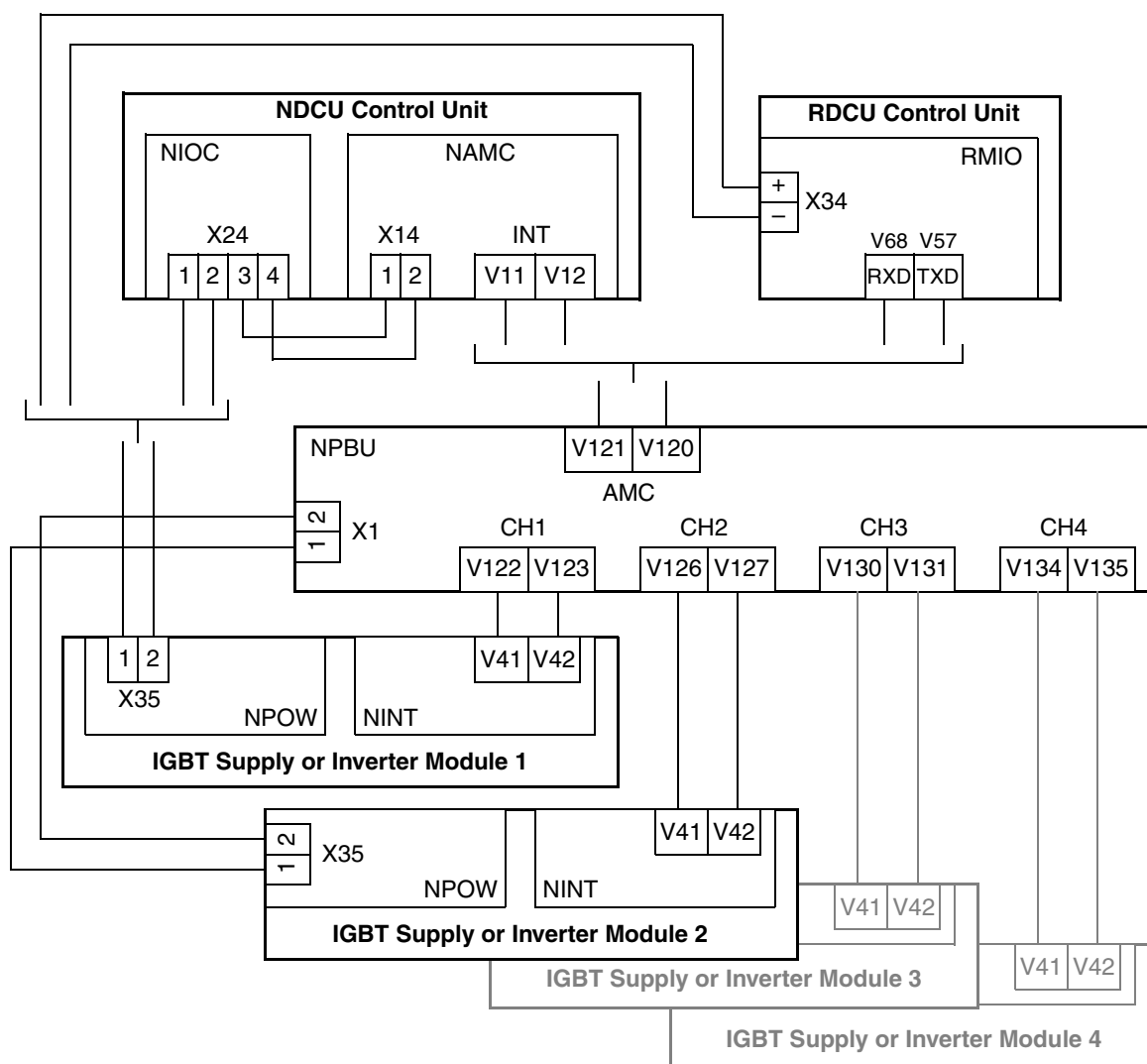
Figure 3-3 Connection of parallel power modules to an RDCU or NDCU control unit through an NPBU optical branching unit.
