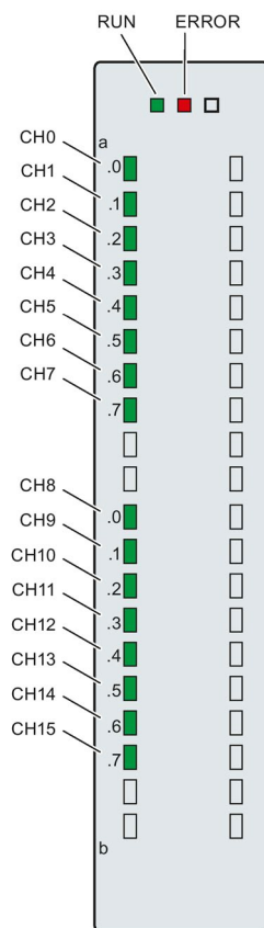
Figure 5-1 LED displays of the module DI 16x24VDC BA
