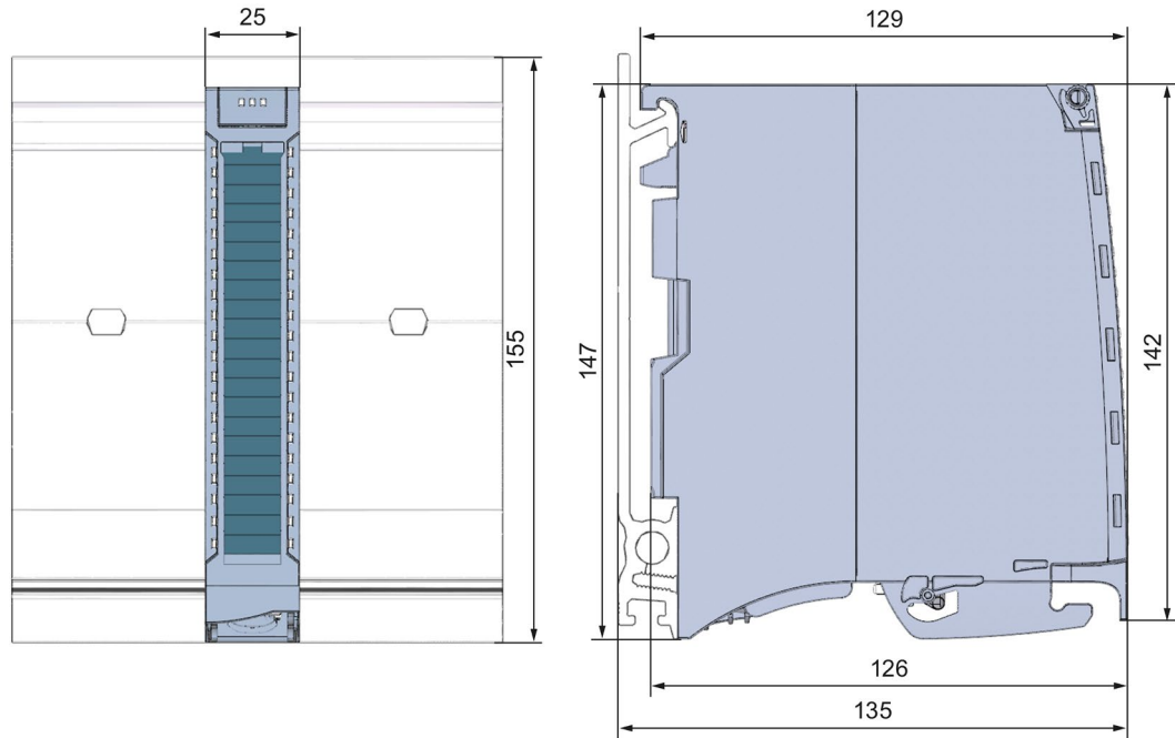
Figure A-1 Dimensional drawing of the DI 16x24VDC BA module
