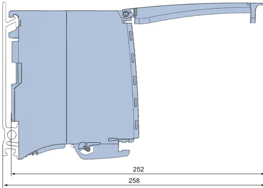
Figure A-2 Dimensional drawing of the DI 16x24VDC BA module, side view with open front cover
