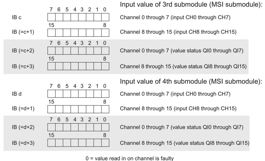
Figure 4-4 Address space for configuration as 1 x 16-channel DI 16x24VDC BA MSI with value status
