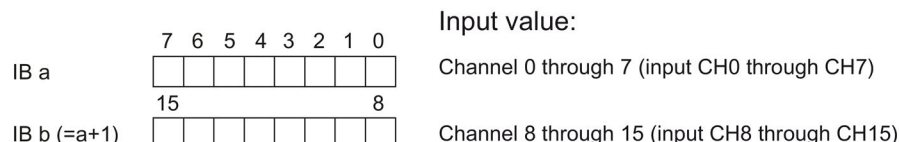
Figure 4-1 Address space for configuration as 1 x 16-channel DI 16x24VDC BA
